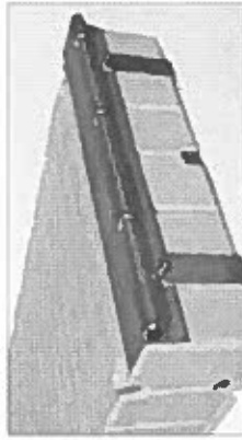
HINGE-TO-FLOAT G200360, G200560 400410, 400460, 400480 Hinged bracket with hardware attaches gangway to dock.
